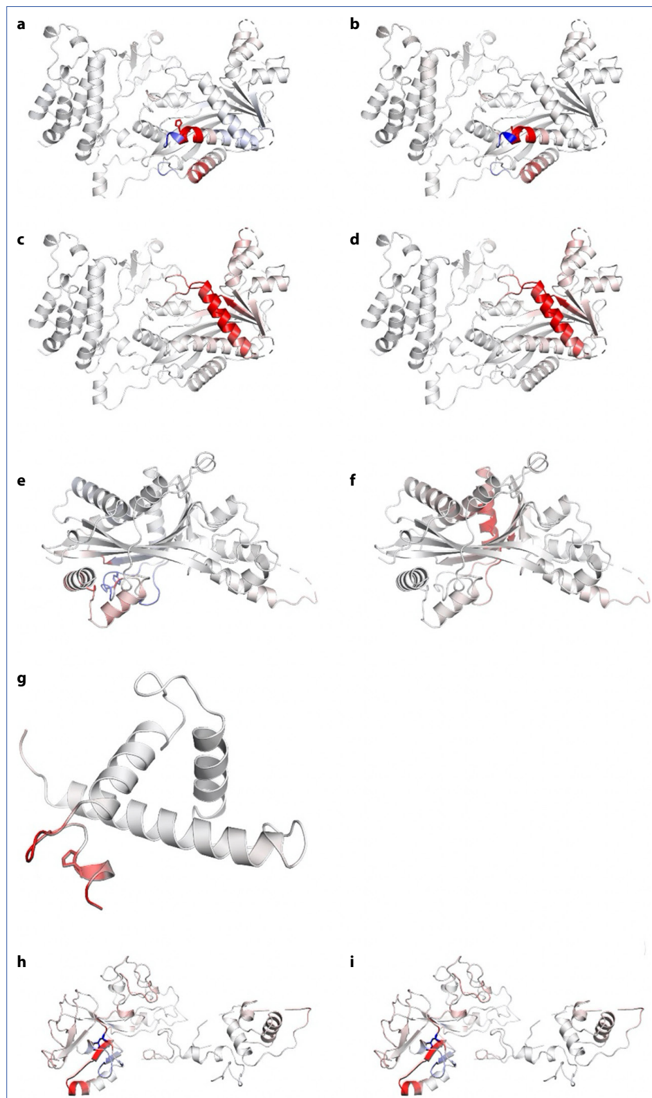
Figure 1. Flexibility visualization of mutations on CREBBP (a-d), EP300 (e-g) and EZH2 (h, i). (a) R1446H; (b) R1446C; (c) Y1503F; (d) Y1503D; (e) H1451Y; (f) Y1467D; (g) L415P; (h) Y641N; (i) Y641F.
